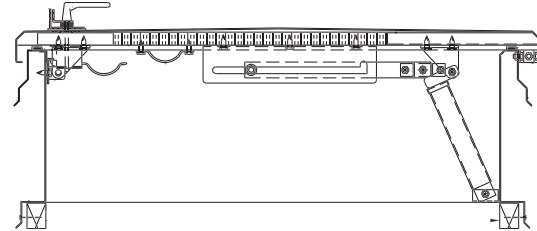
Curb Mounted Roof Hatch
